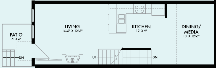
First Floor
